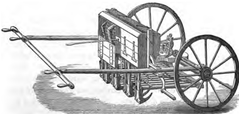
BEDFORDSHIRE DRILL.
